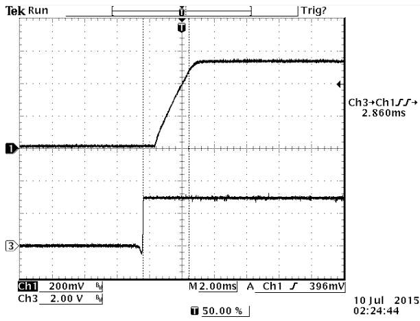
Figure 18. Start up time at full load, 12VDC input 0.6VDC/30A output and Ta=25 °C
